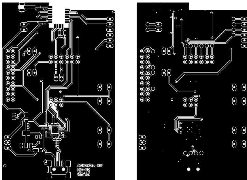
Figure 15: Top & bottom Layer
