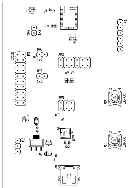
Figure 14: Assembly diagram
